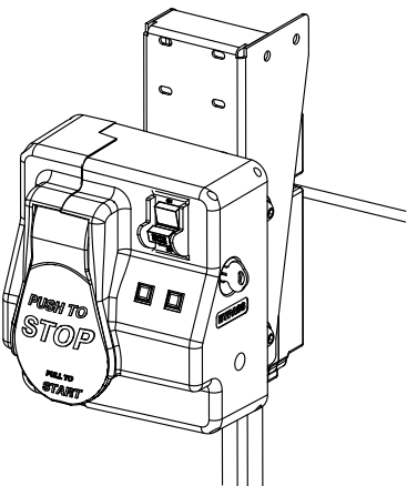
switch box assembly (connected to the saw by electrical cables)
