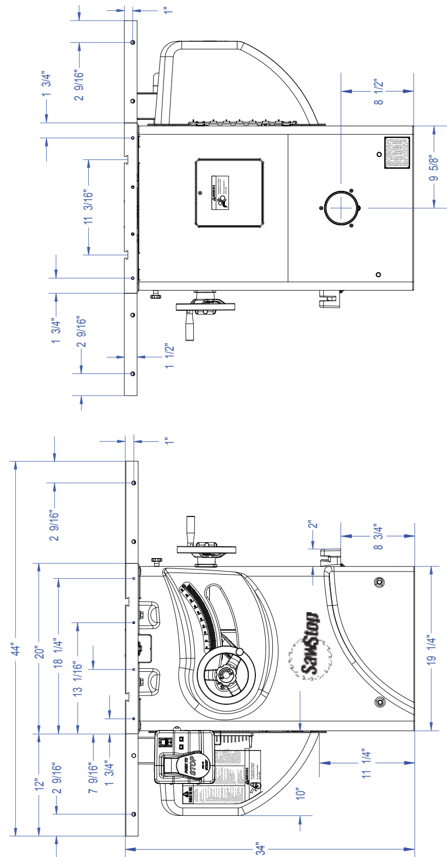
Front View
