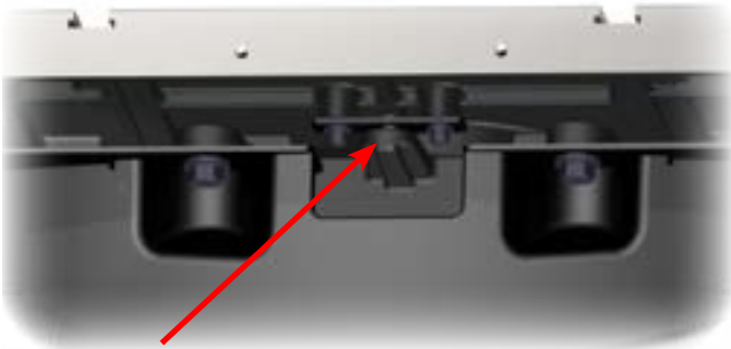
The pivot pin is pressed into this boss
